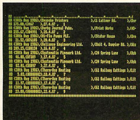
Figure 4. Multi-macro file in View
